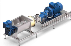
Screw Pumps
